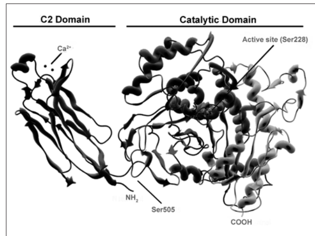
Figure 1. Ribbon diagram of cPLA 2 α. The C2 domain on the left mediates interaction of the enzyme with membranes via binding of two Ca 2+ atoms. The active site Ser 228 on the catalytic domain is highlighted, as is the phosphorylation site Ser 505.
